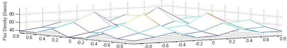
Flux Density at 0.8 cm Above Surface
