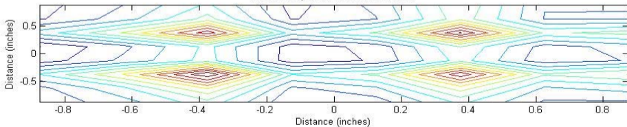
Flux Density at 0.8 cm Above Surface
