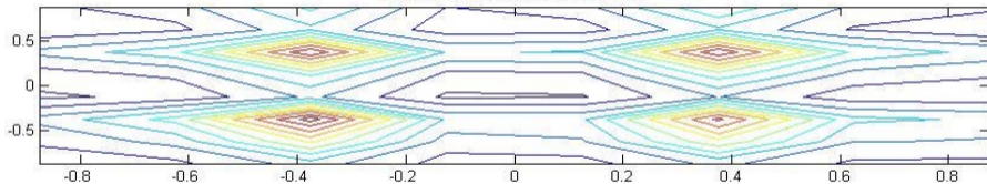
Flux Density at 0.8 cm Above Surface
