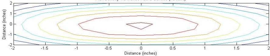
Flux Density 1.5 inches Above Surface (kGauss)
