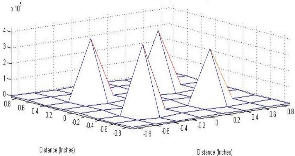
Force Index at 0.4 cm Above Surface (Gauss*Gauss/cm)
