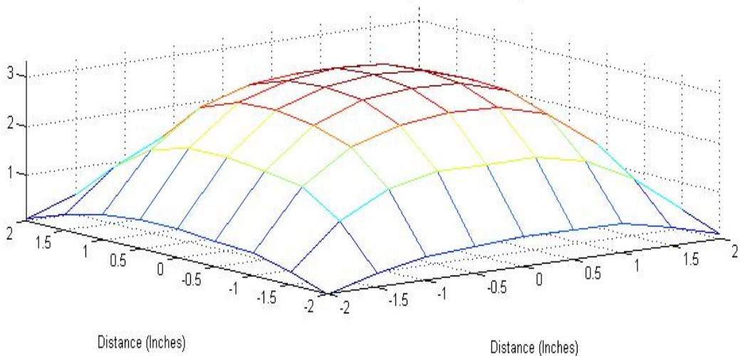
Force Index at 1 Inch Above Surface (kGauss*kGauss/inch)
